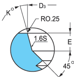
Detail X
