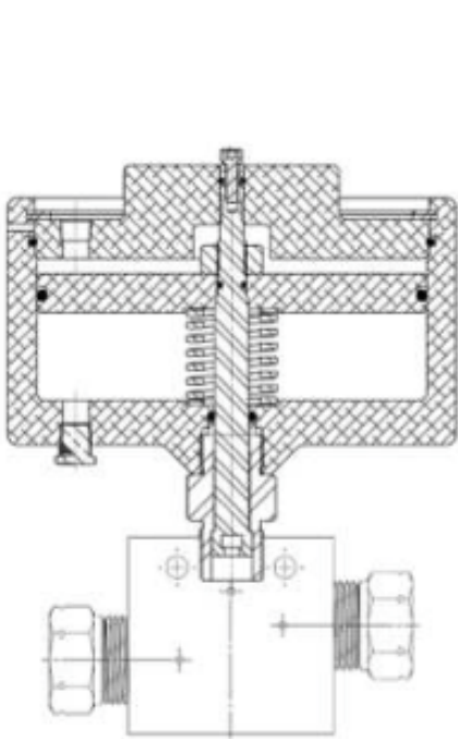
Normally Open (Air-to-Close)
